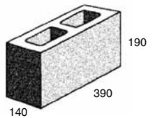
15.01 Hollow - full length
