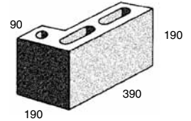
10.25 Hollow - corner return
