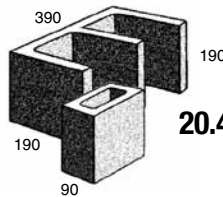
10.02 Hollow - quarter
