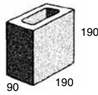
10.03 Hollow - half
