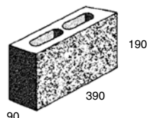
10.121 Hollow - full length
