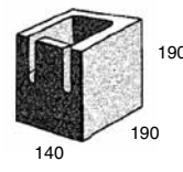
15.43 Closed end - half
