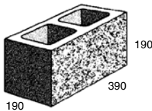
20.121 Hollow - full length
