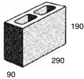
10.02 Hollow - three quarter
