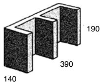
15.45 Clean-out stretcher
