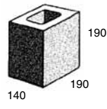
15.03 Hollow - half
