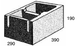
30.41 Closed end
