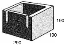
20.02 / 30.43 Hollow - half / Closed end - half
