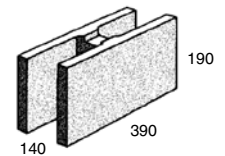
15.48 'H' block
